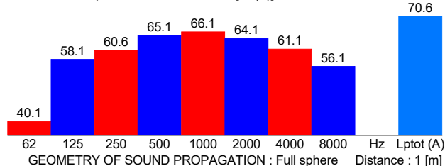
Lp - SOUND PRESSURE [dB(A)]
