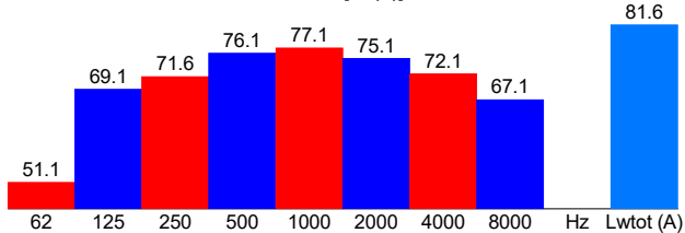
Lw - SOUND POWER [dB(A)]
